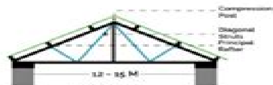
Fink Truss
