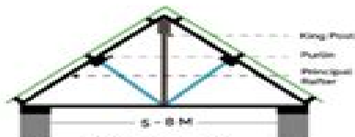
King Post Truss
