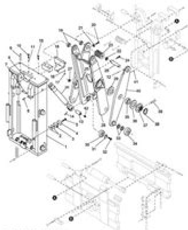
33 Reach - Tilt with Sideshift, RR only
