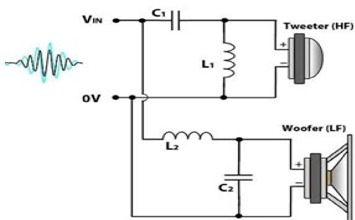
2-way car stereo speaker crossovers
