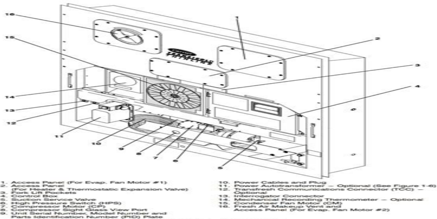
Figure 1-1. Refrigeration Unit – Front
