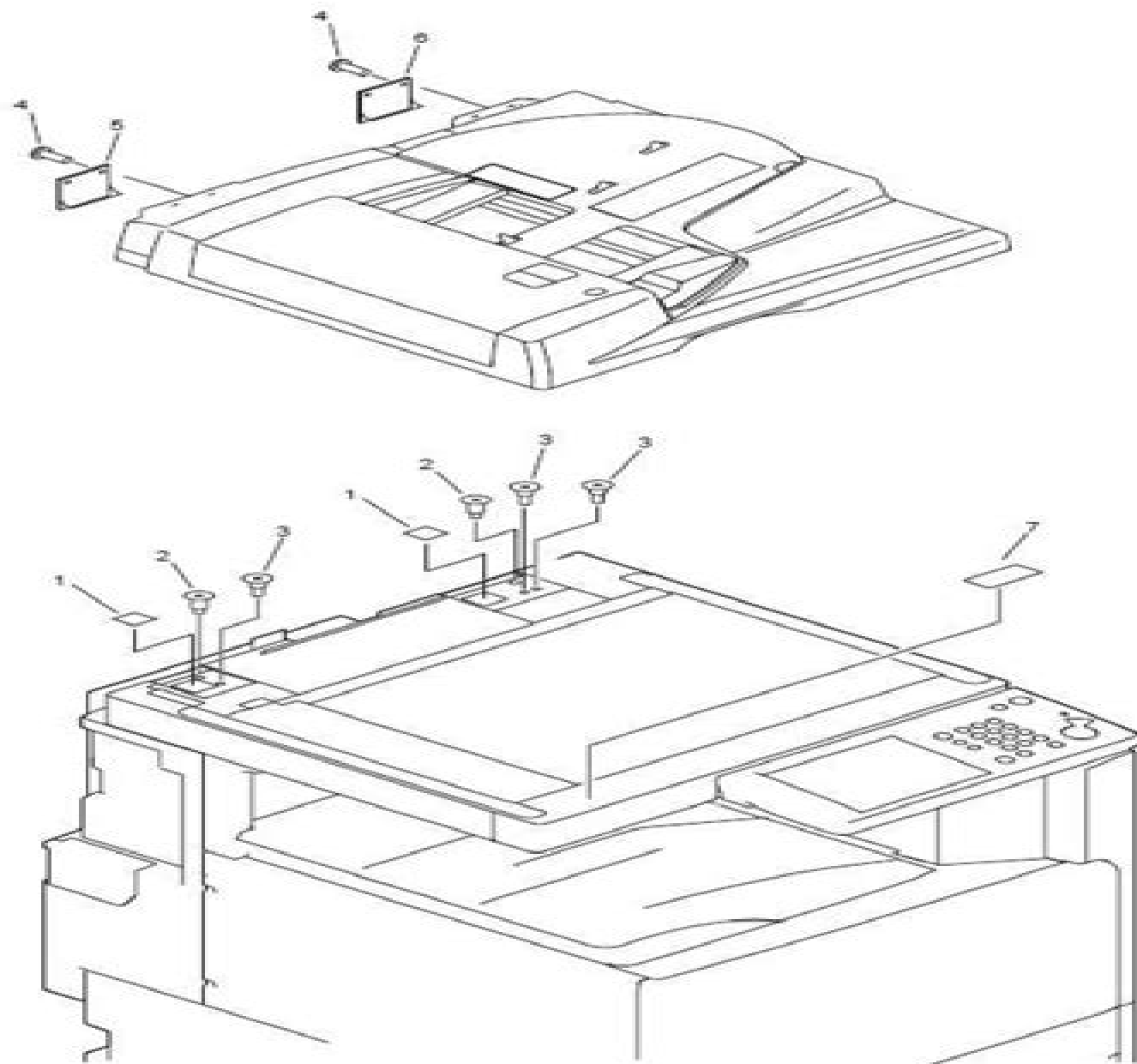
FIGURE 160 DADF MOUNTING HARDWARE
