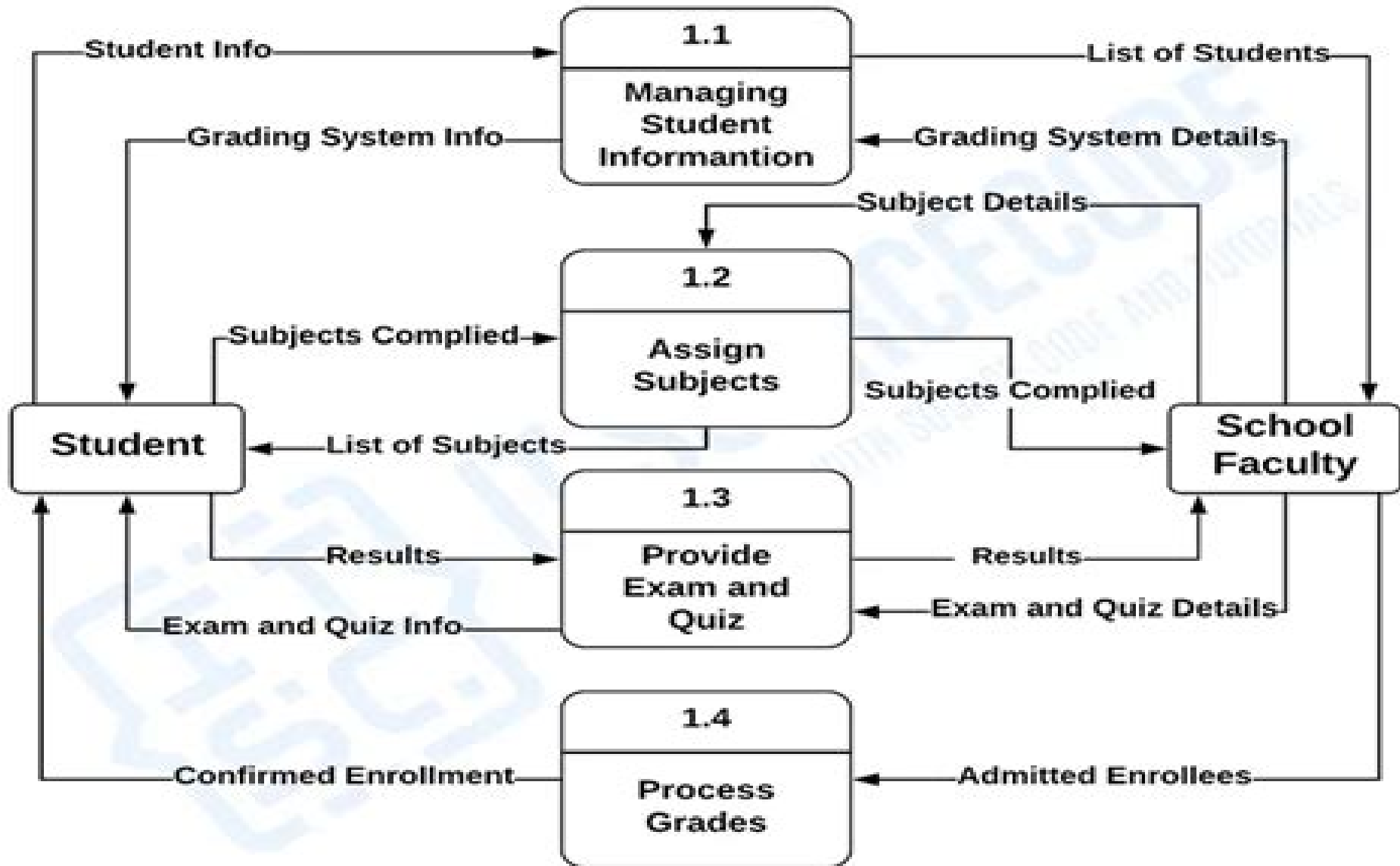
DATA FLOW DIAGRAM LEVEL 1
