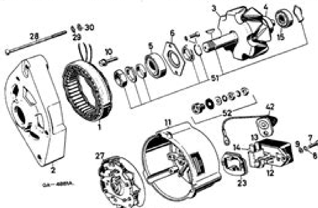
Illustr. 12 "Q1" alternator, with piggy-back voltage regulator and load dump diode
