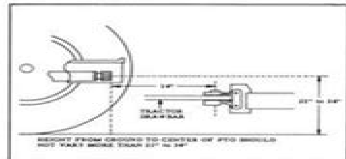
Figure 15. Hitch Dimensions
