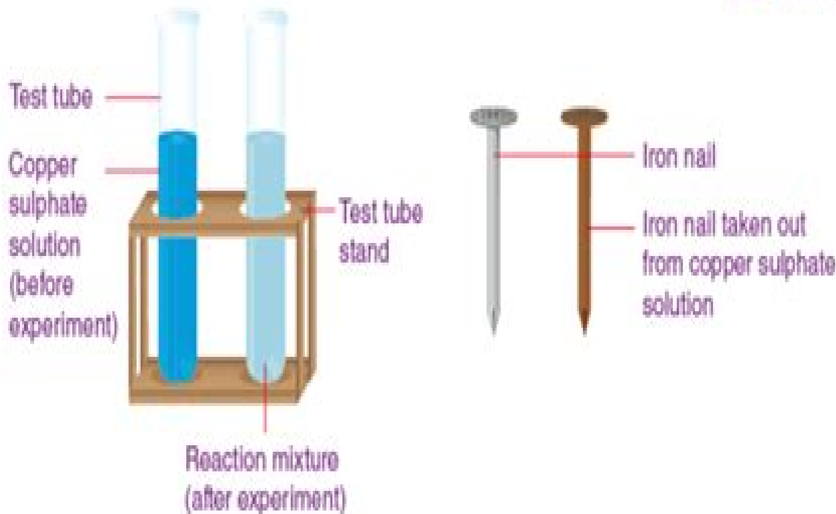
Fig: Single displacement reaction – Iron nails with copper sulphate solution
