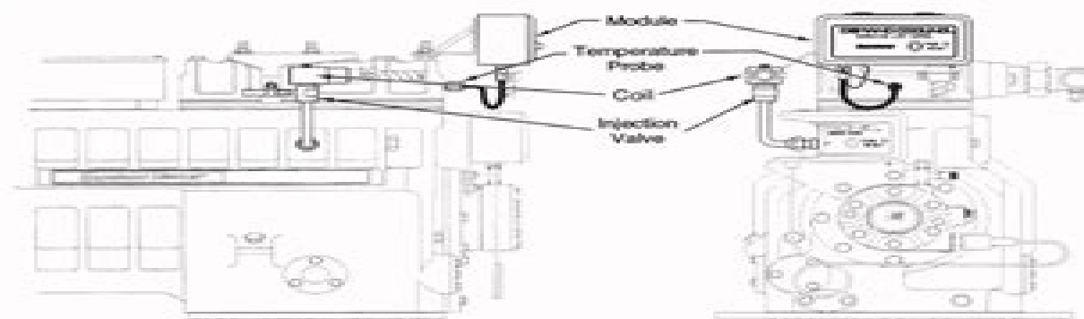
Figure 1 – Demand Cooling System
