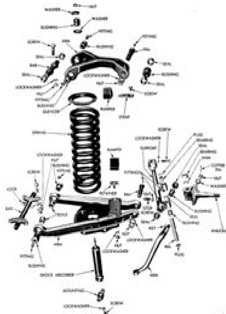
Fig. 1-Front Wheel Suspension
