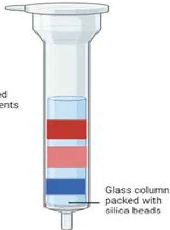
Column chromatography
