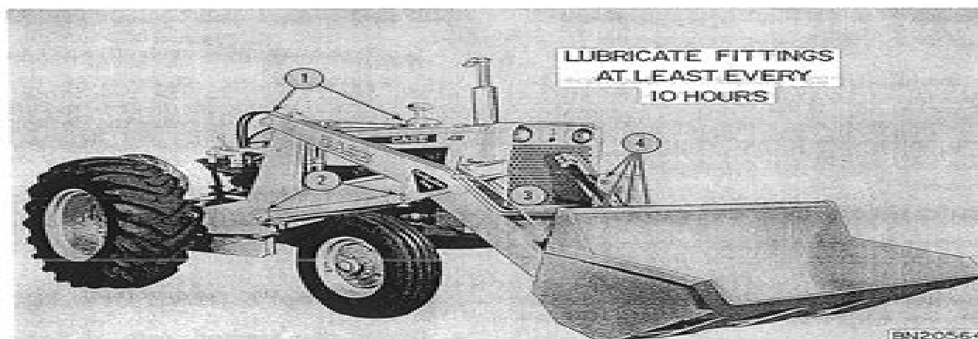
Figure 3 - Loader Pressure Fittings
