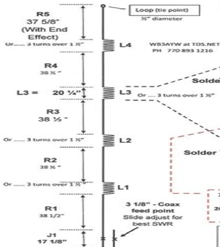
Fig 1 J-fed 5-element collinear 2 Meter Antenna by WB3AYW
