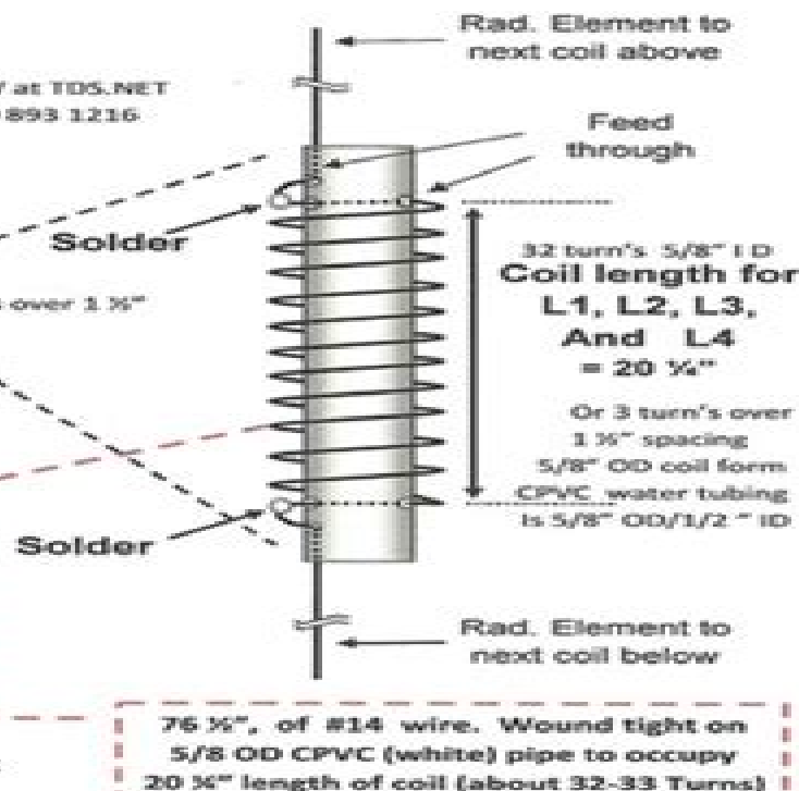
Fig 2 Construction detail for L1, L2, L3 and L4 (all)
