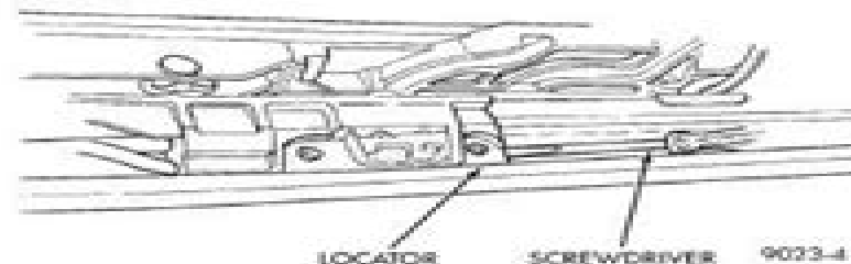
Fig. 4 Removing Cable Drive Locator
