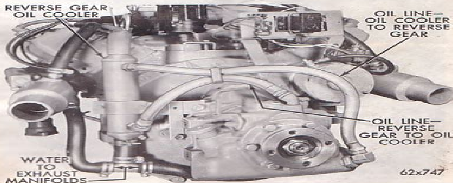
Figure 12—Reverse Gear Oil Cooler Connections Models 318
