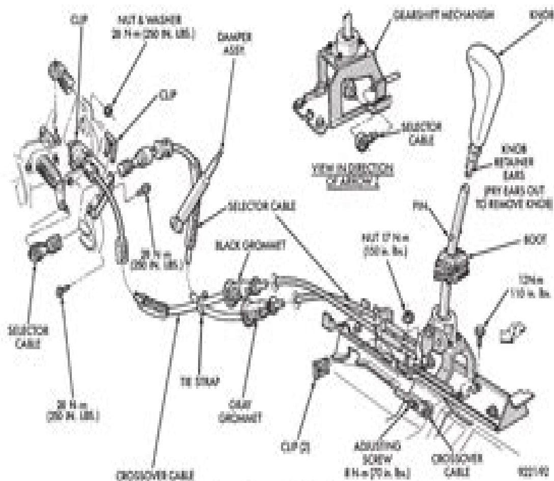
Fig. 1 Gearshift Mechanism
