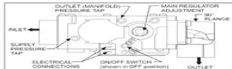
FIGURE 29: Gas Valve
