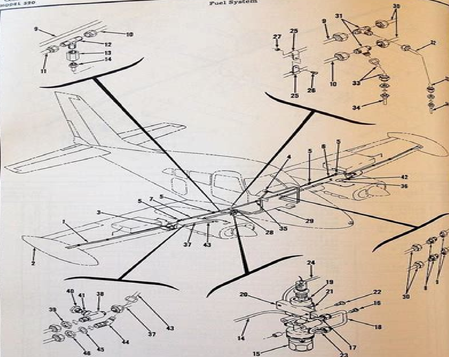
Figure 137. Fuel System Installation
