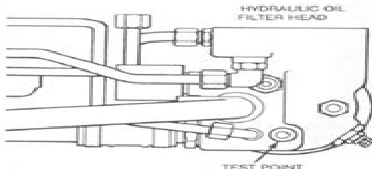
Fig. 171—Top view of hydraulic oil filter head showing charge and lubrication pump pressure test port.
