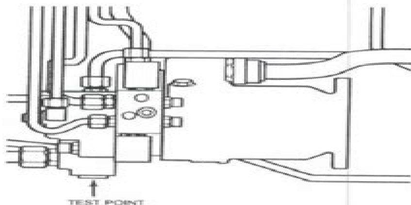
Fig. 173—Install pressure gauge at test point shown when checking low standby pressure or pump maximum pressure.
