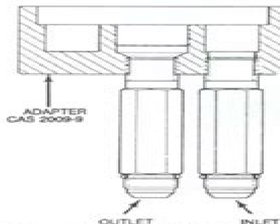
Fig. 172—Flowmeter adapter (CAS-2009-9) installed in place of hydraulic oil filter element to test charge pump flow.
