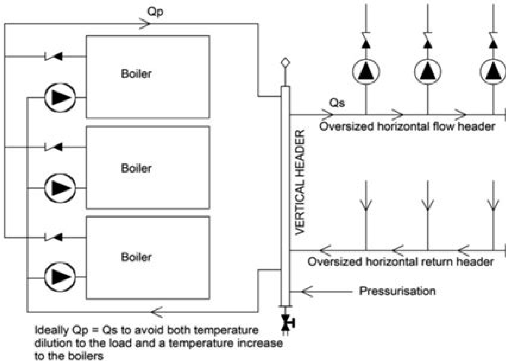
Figure 3: Recommended system configuration
