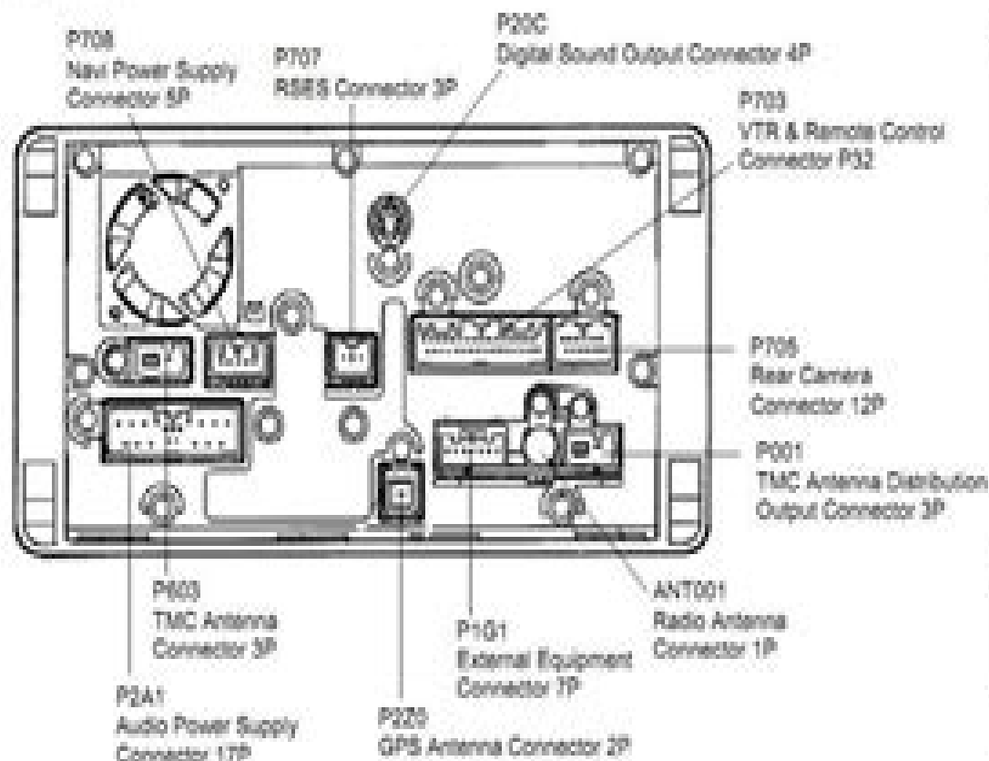
Audio Power Supply Connector 17P
