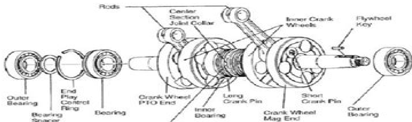
Crankshaft Exploded View and Nomenclature
