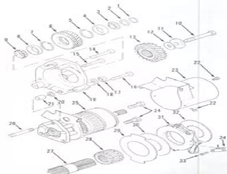
Fig. 15—Exploded view of front drive axle clutch, drive gears and components.
