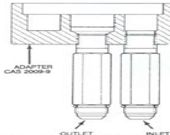
Fig. 172—Flowmeter adapter (CAS-2009-9) installed in place of hydraulic oil filter element to test charge pump flow.
