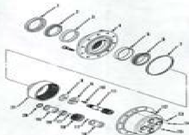
Fig. 8—Exploded view of wheel hub and planetary unit used on front drive axle.
