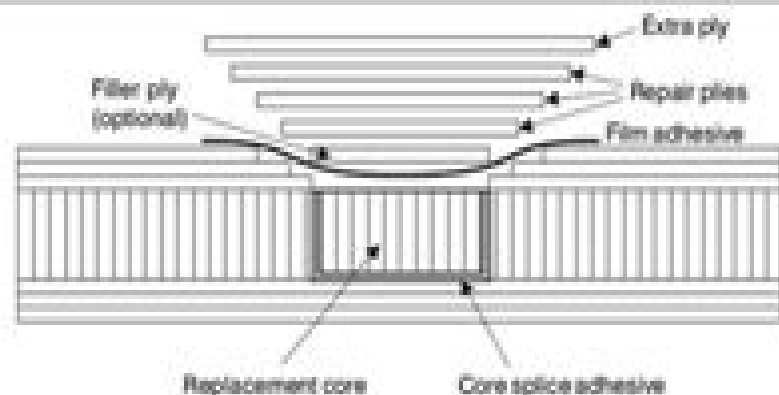
Stepped repair
