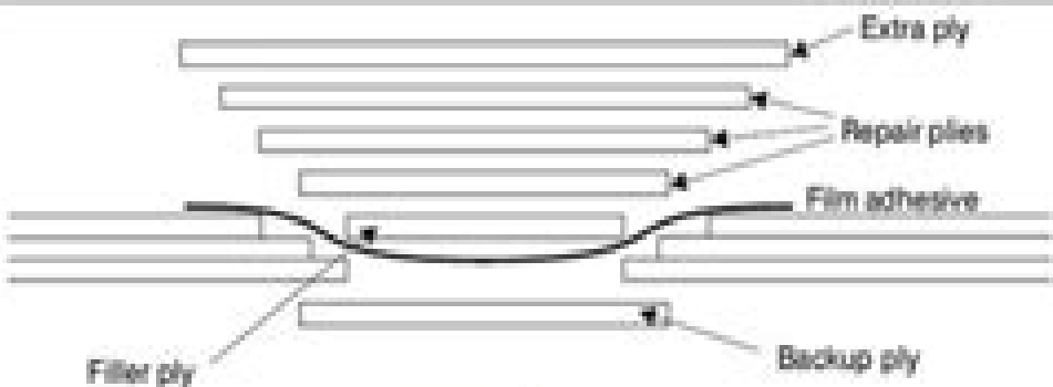
Stepped repair
