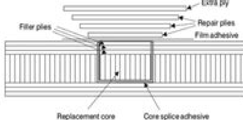
Patch repair
