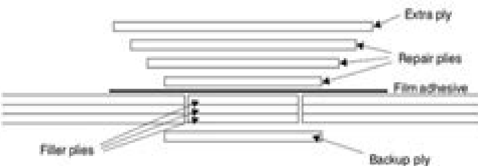
Patch repair
