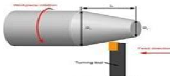
Taper Turning
