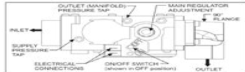
FIGURE 29: Gas Valve
