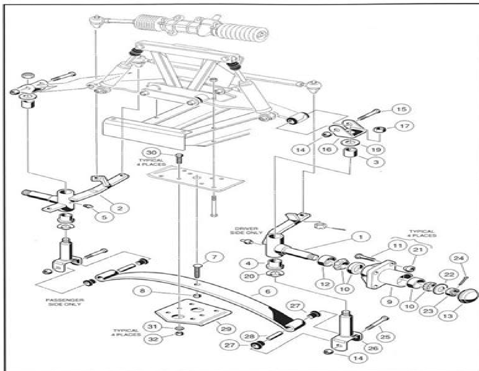
Figure 7-21 Two-Wheel Brake Vehicle – Lower Portion
