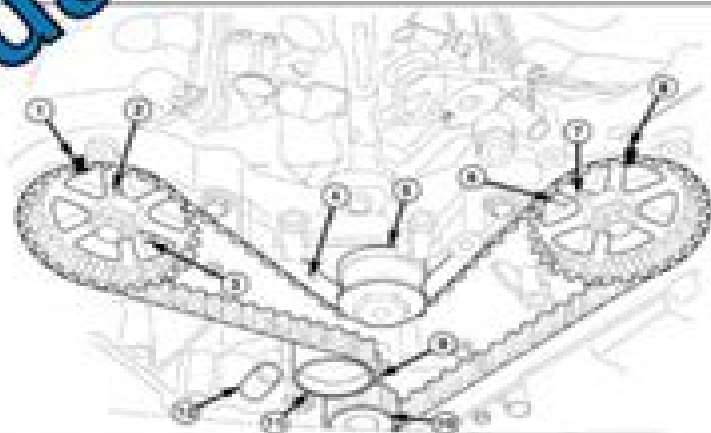
TIMING GEAR ALIGNMENT
