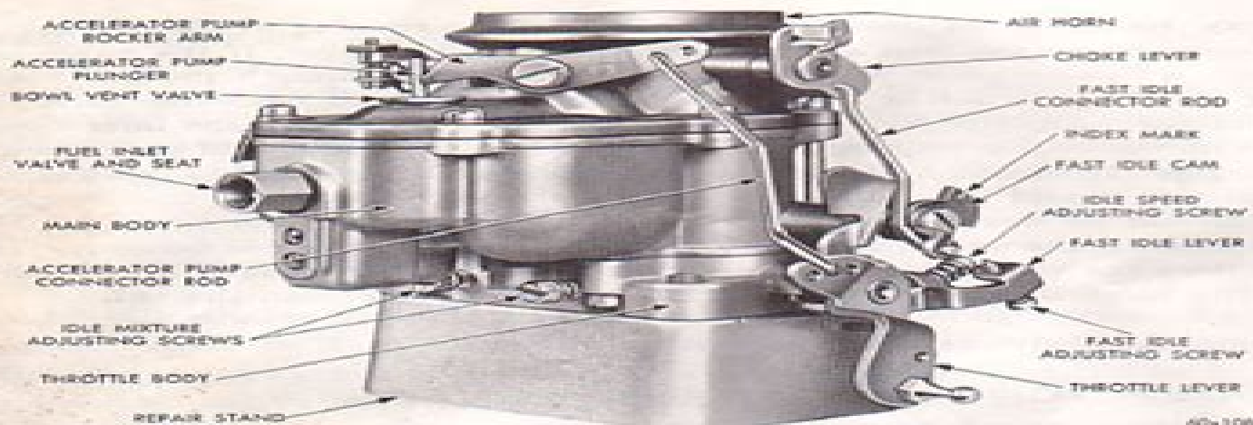
Figure 25—Carburetor Assembly BBD Series Used on Models M-318A
