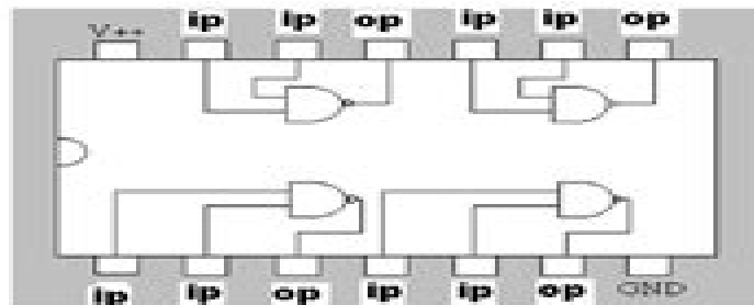
Fig (i) Pin diagram of NAND Gate (IC 7400) and logic symbol
