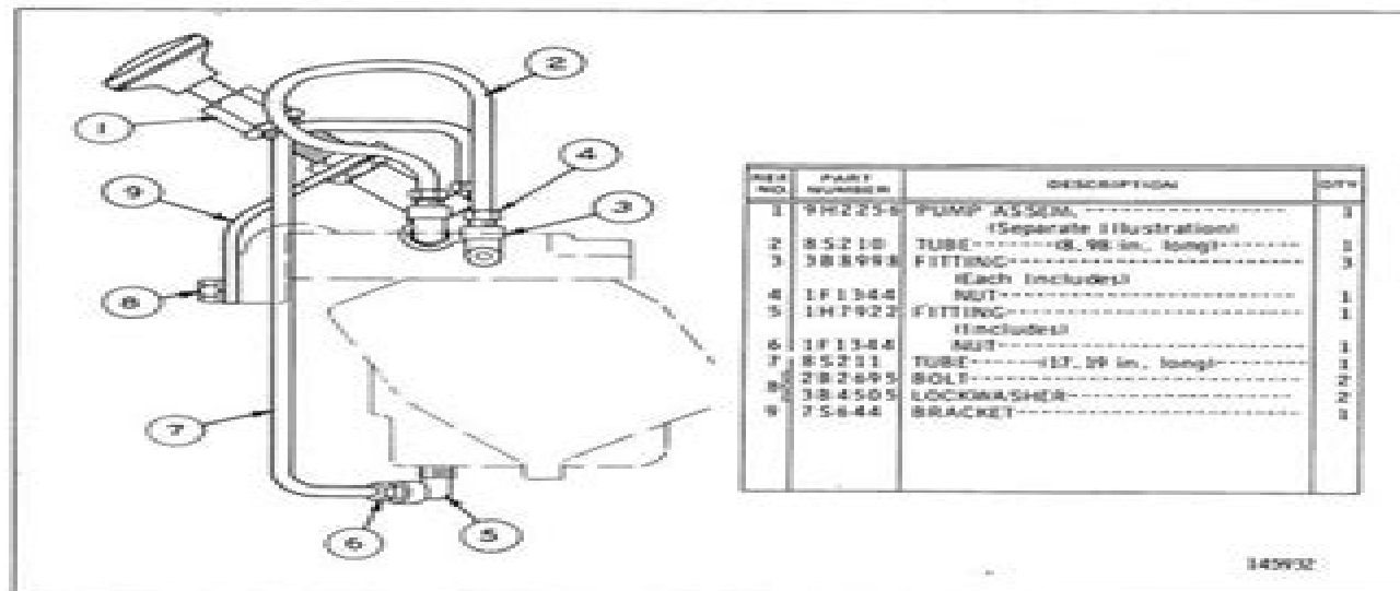
FUEL PRIMING PUMP (5S2100 N/S) 9H2256 Pump parts are shown on Page 36A.
