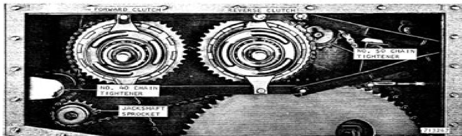
Figure 11 - Drive Chains, Clutches and Sprockets
