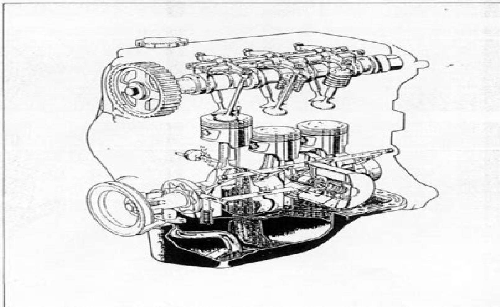
FIG. 1A — 2 ENGINE LUBRICATION
