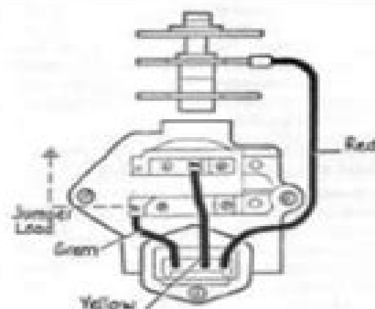
Fig. 80—Schematic view of 8TRD regulator.
