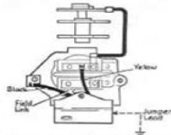
Fig. 81—Schematic view of 14TR regulator.
