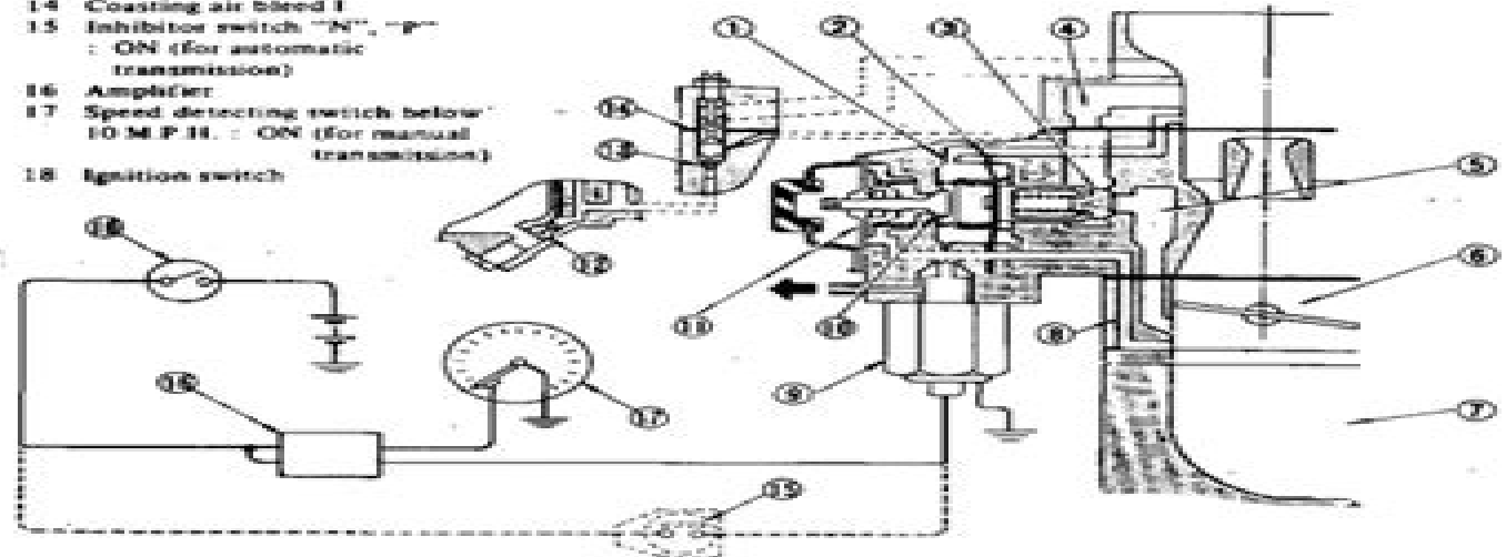
Fig. EF-31 Schematic drawing of B.C.D.D. (Non-California models)
