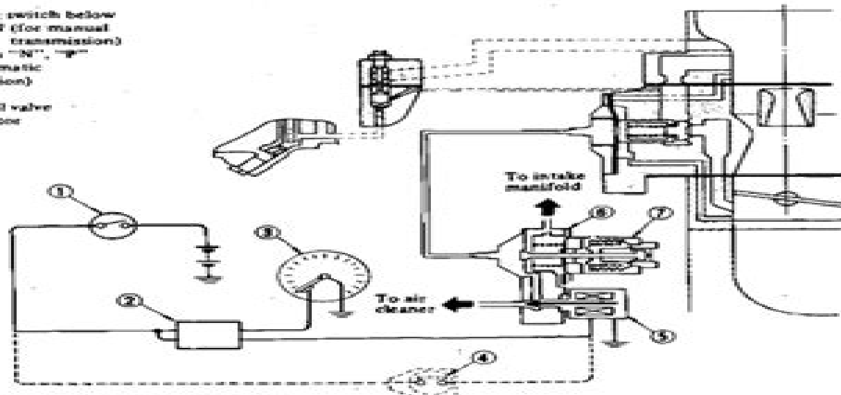
Fig. EF-32 Schematic drawing of B.C.D.D. (California models)
