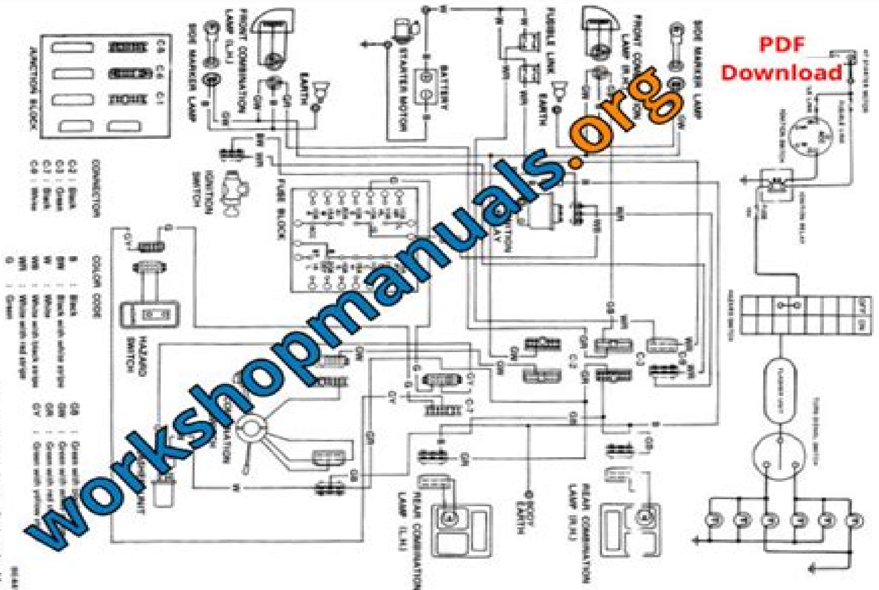
Fig. 10.17 Control diagram for two output loops
