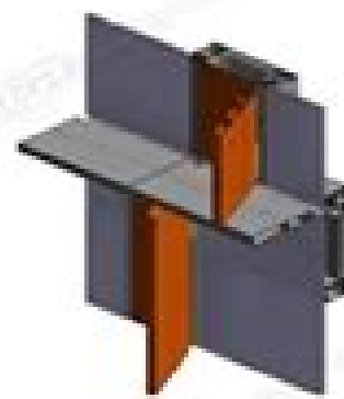
3. INTERMEDIATE MULLION & PANEL, WITH FIN - 3D VIEW
