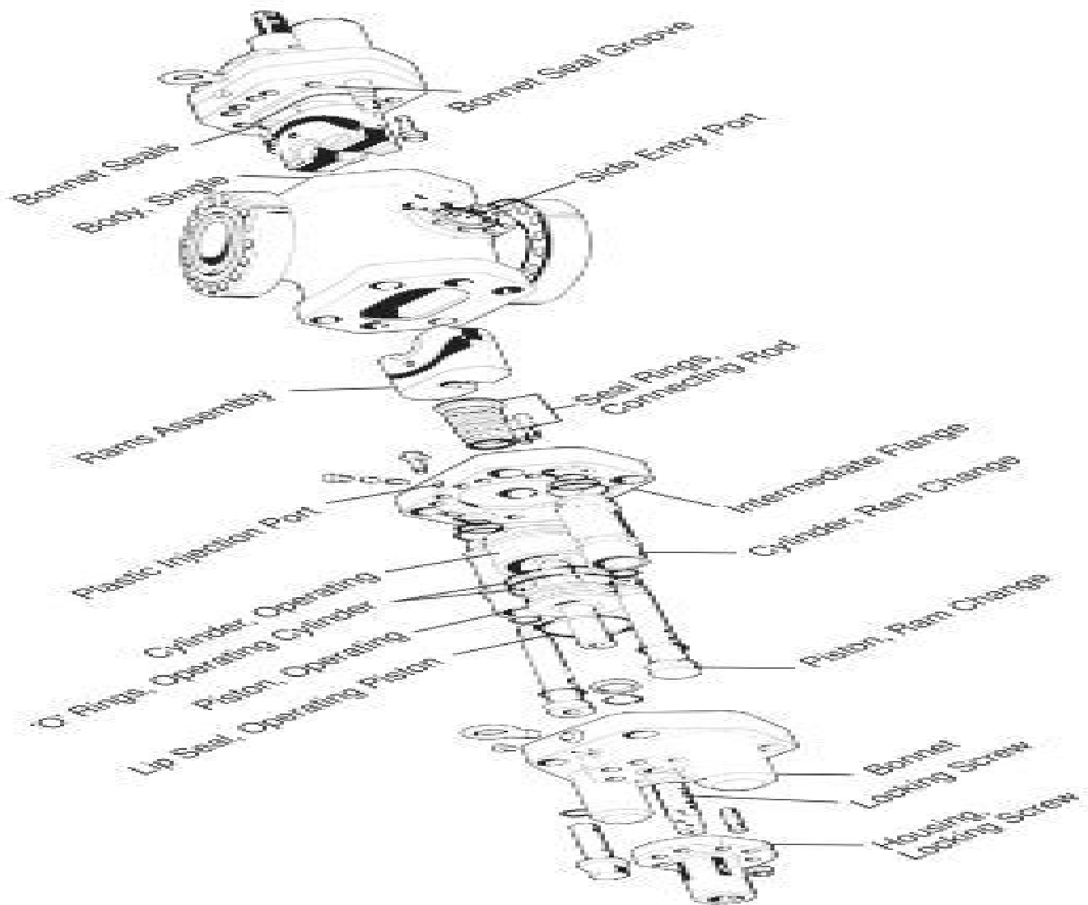
Figure 6.1.3 Figure Cameron U - Type BOP
