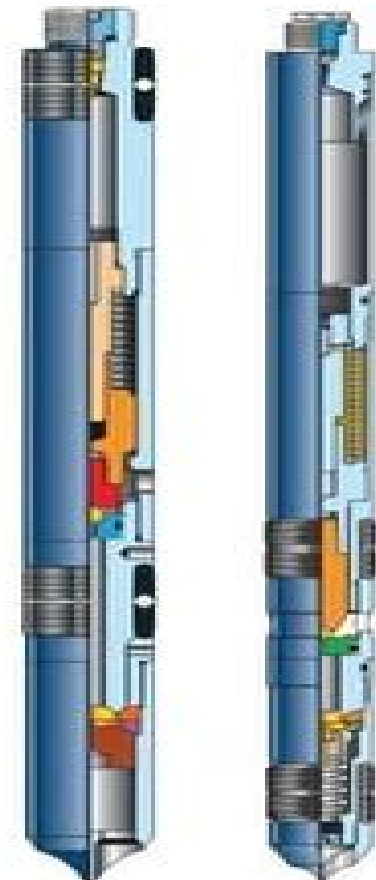
BK series gas lift valve (left) and R-20-G2 series gas lift valve (right)
