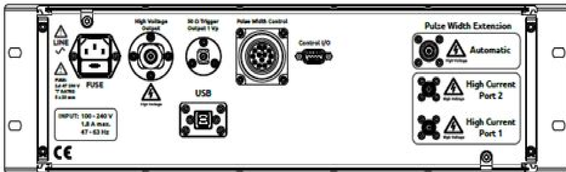
Figure 3: CMTI-8010A schematic rear view
