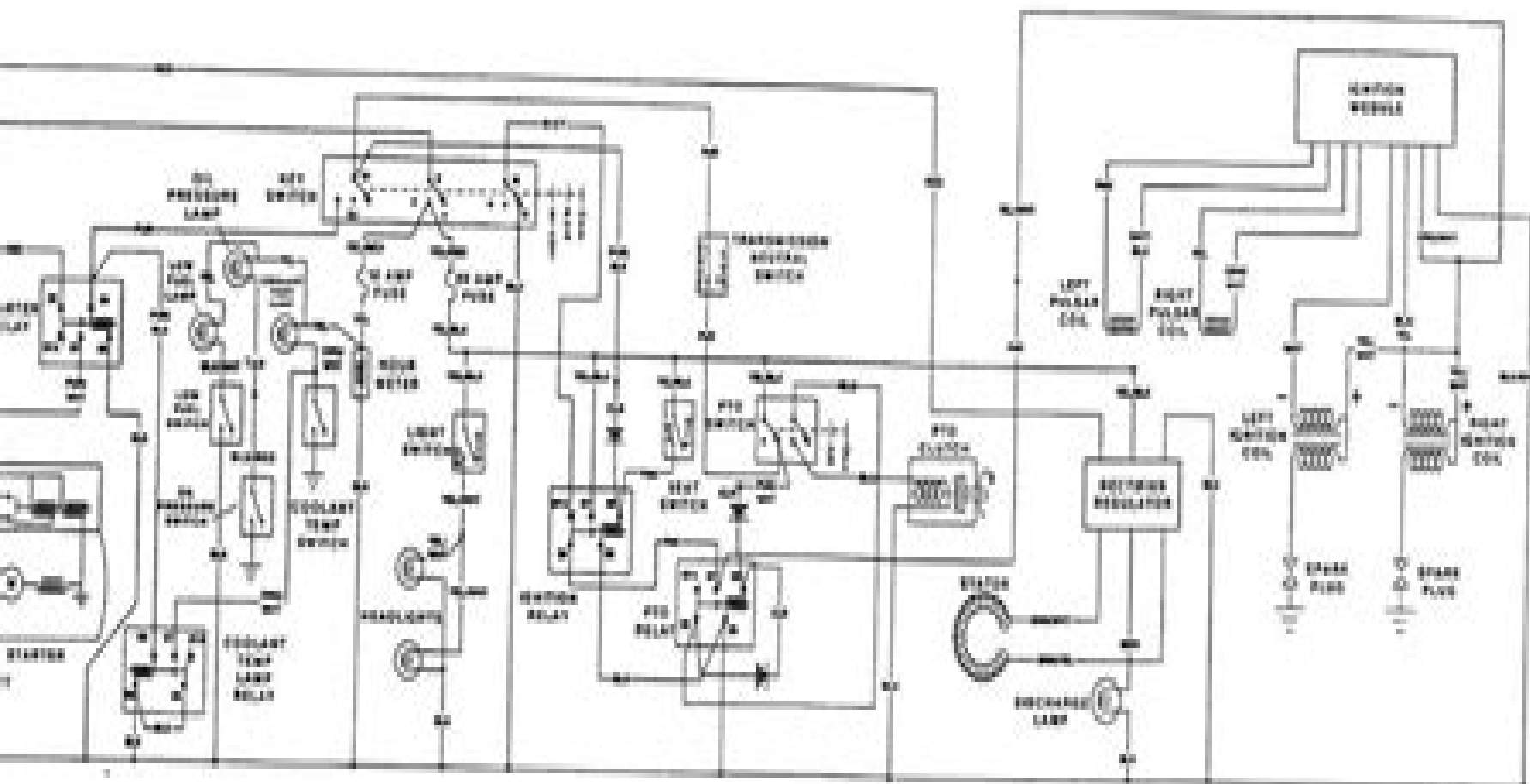
—Wiring diagram for Model 285 with carbureted engine. Refer to Fig. JD5-10 for fuel injection wiring diagram.
