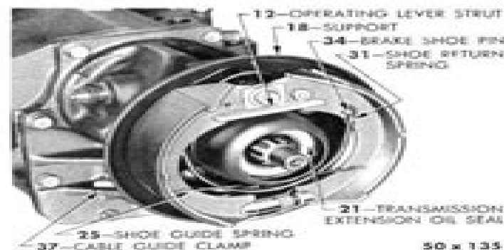
Fig. 22 — Internal Expanding Hand Brake
