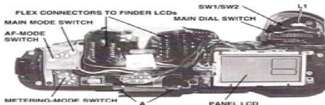
FIG. 1 TOP VIEW
