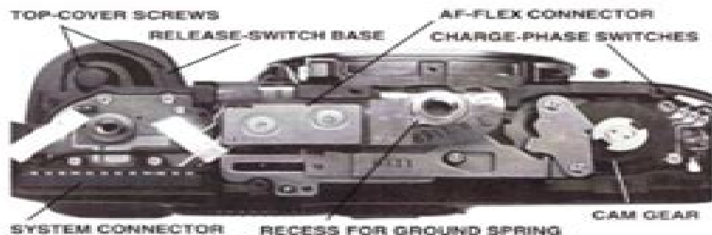
FIG. 2 BOTTOM VIEW
