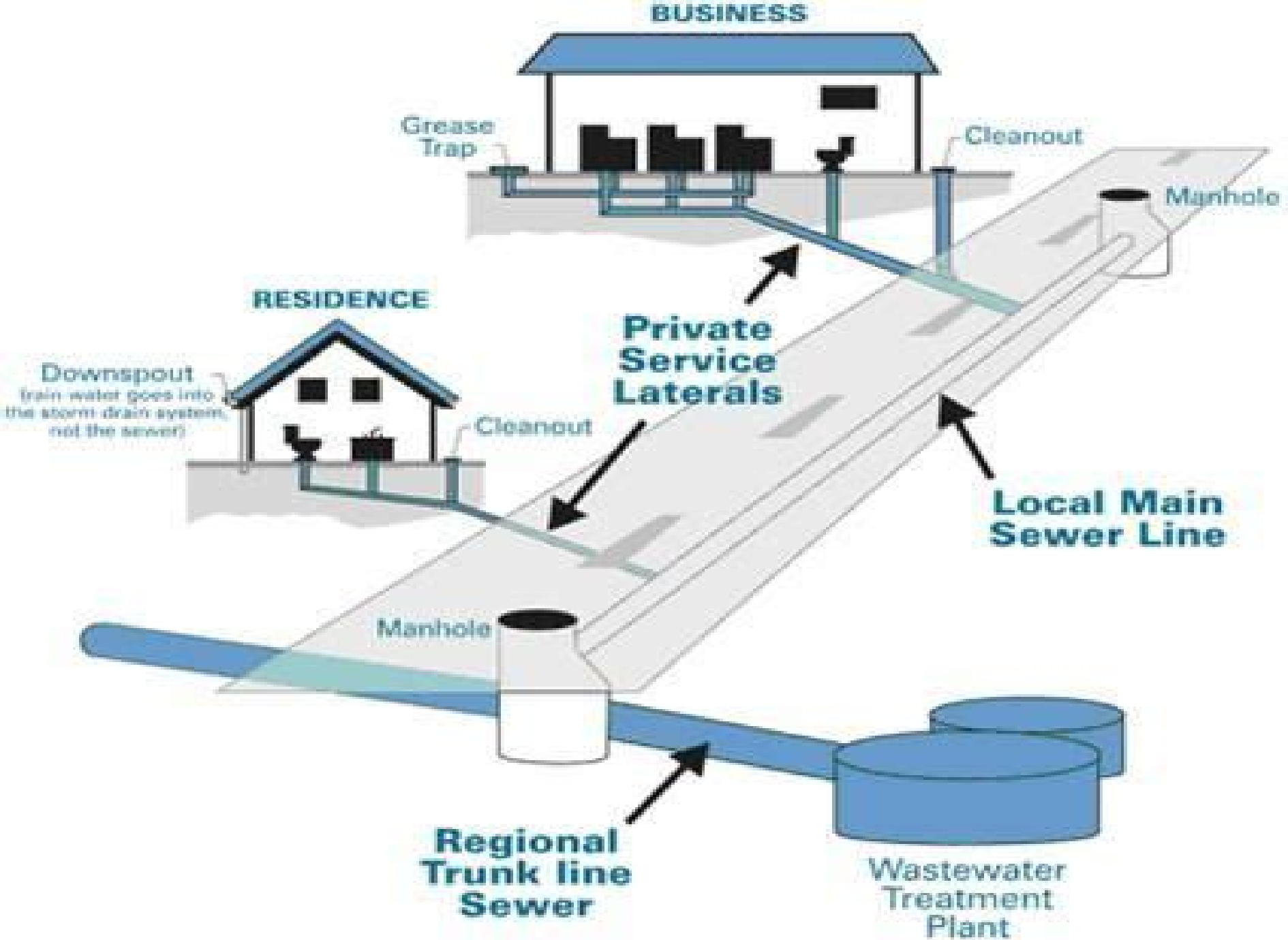
Diagram of a sanitary sewer system
