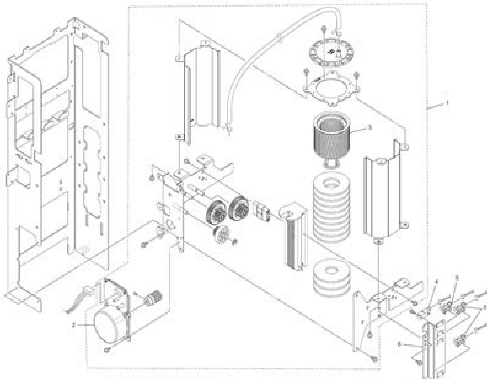
Fig.28 Bellows
