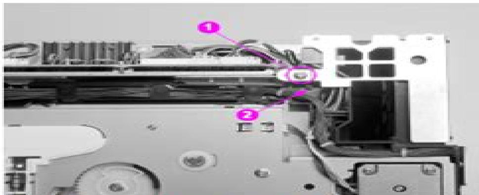
Figure 6-38 Large fan removal and replacement (2 of 2)
