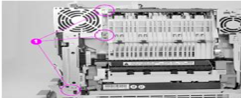
Figure 6-37 Large fan removal and replacement (1 of 2)
