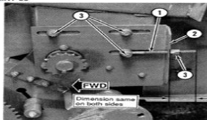
FIGURE MNT-31. FLOOR BELT ADJUSTMENT
